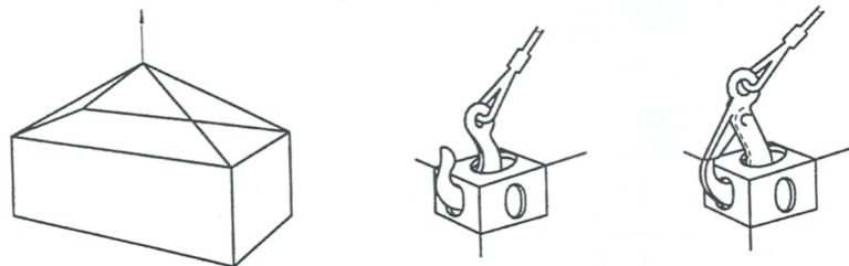
picture 2 – lifting by top ISO corners
